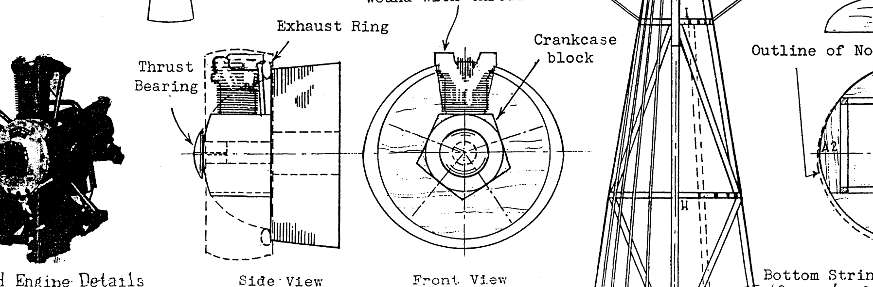
Leblond Engine Details
