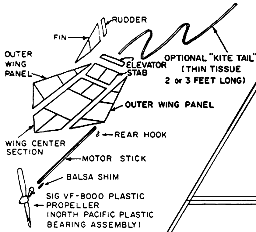
EXPLODED VIEW
