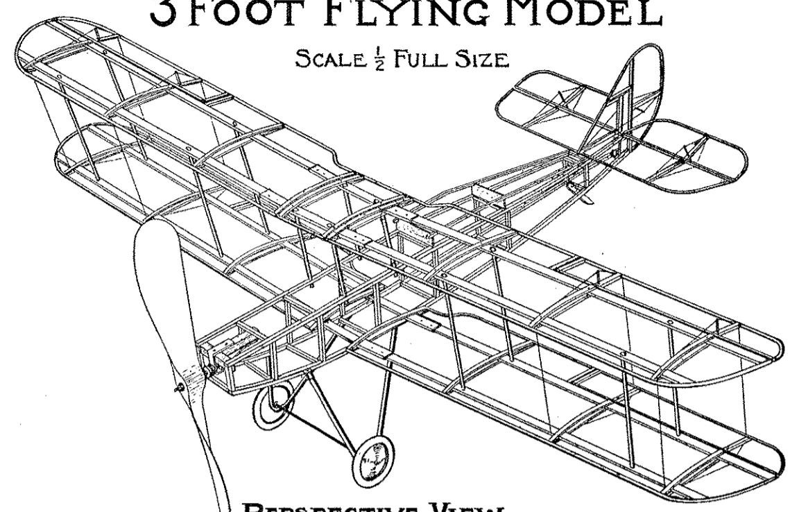
PERSPECTIVE VIEW COVERING AND COWLING OMITTED
