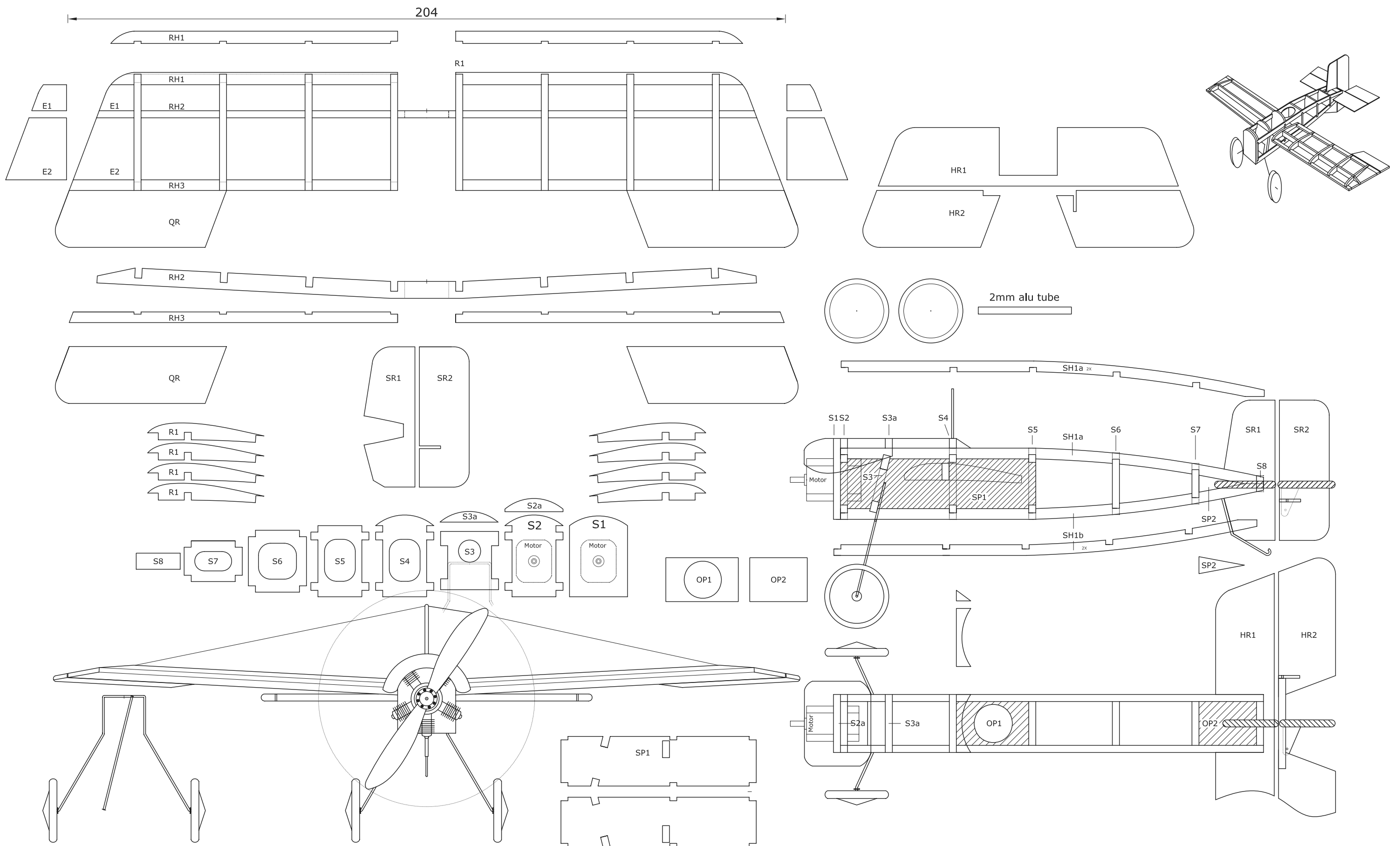
Pionero Pistachio Scale by Arno Diemer All Wood is 2mm Balsa Wood unless stated otherwise
