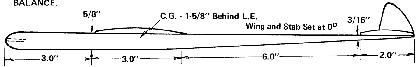
Fuselage is 5/8" x 1/8" x 14" Blank - Stringy Med. Stock - Drawn Half-Size
