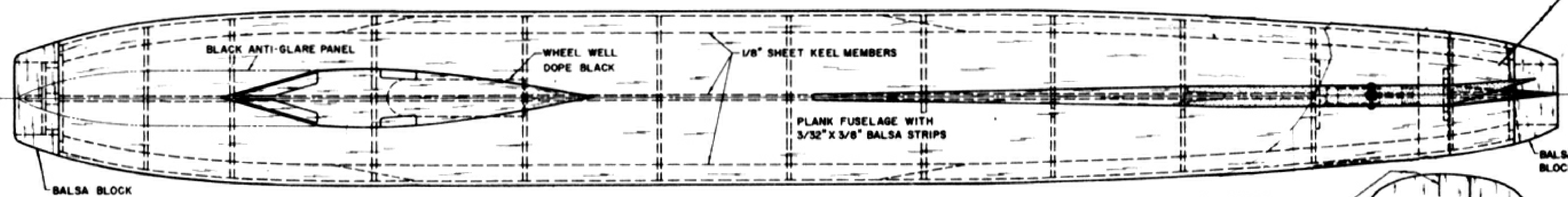
DOUGLAS D558 SKYSTREAK DESIGNED BY FRANK W. BEATTY
