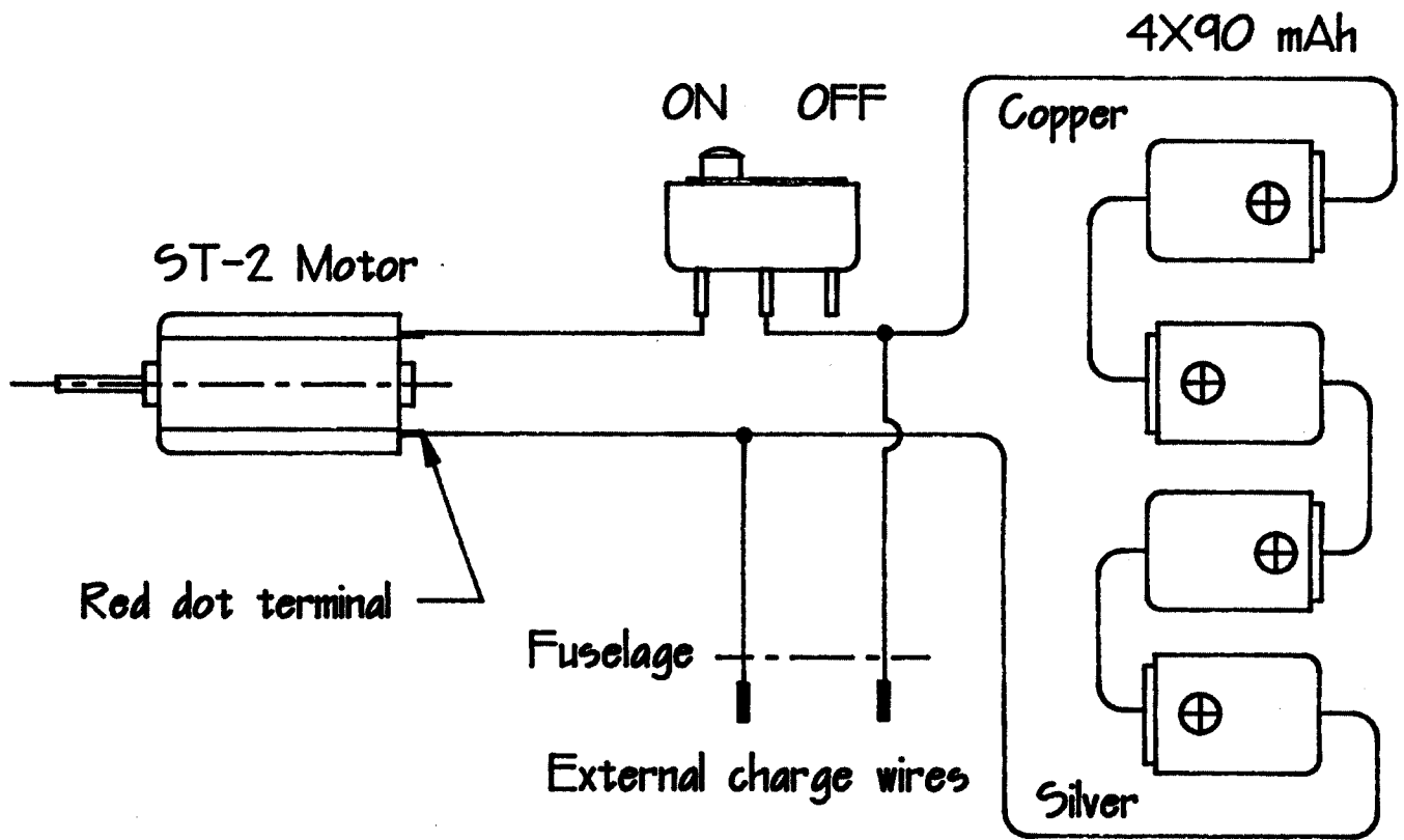
Norseman Wiring Diagram
