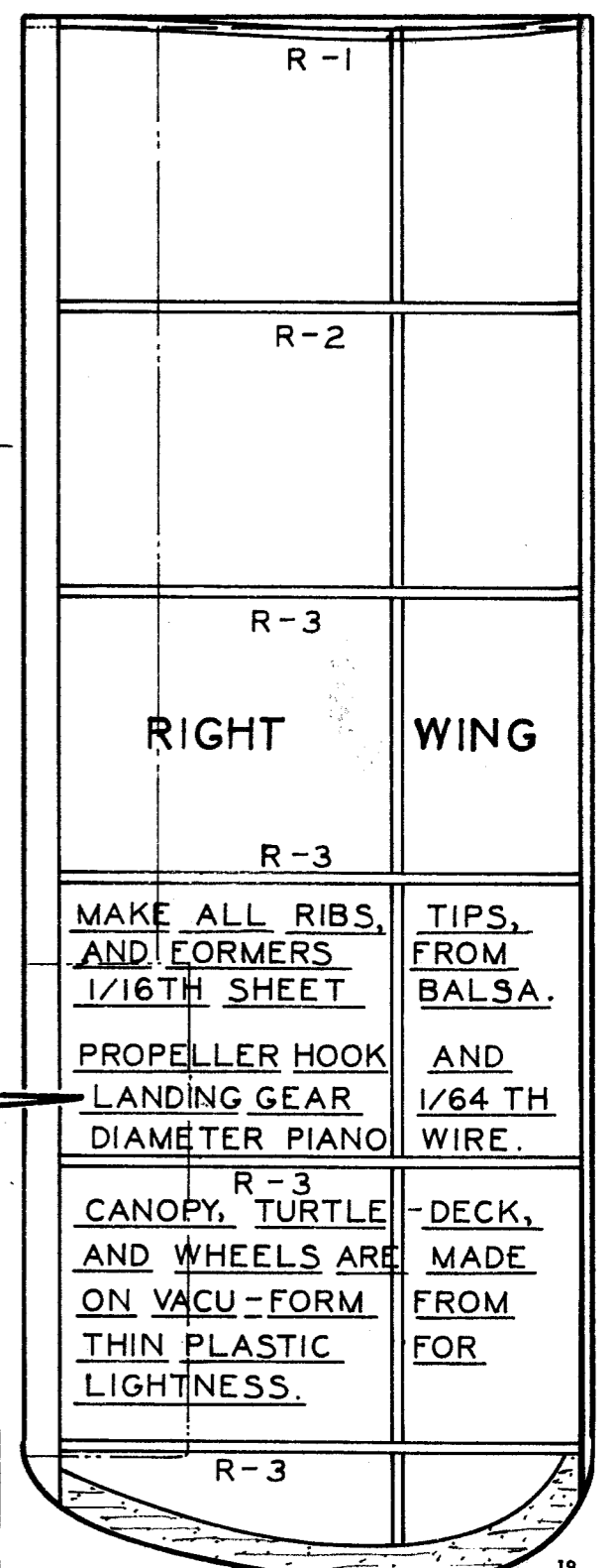
LOCKHEED LITTLE DIPPER BY Walt Mooney 2-22-65
