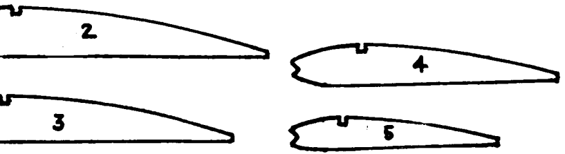
W2 - W5 wing ribs from 1/32'' sheet
