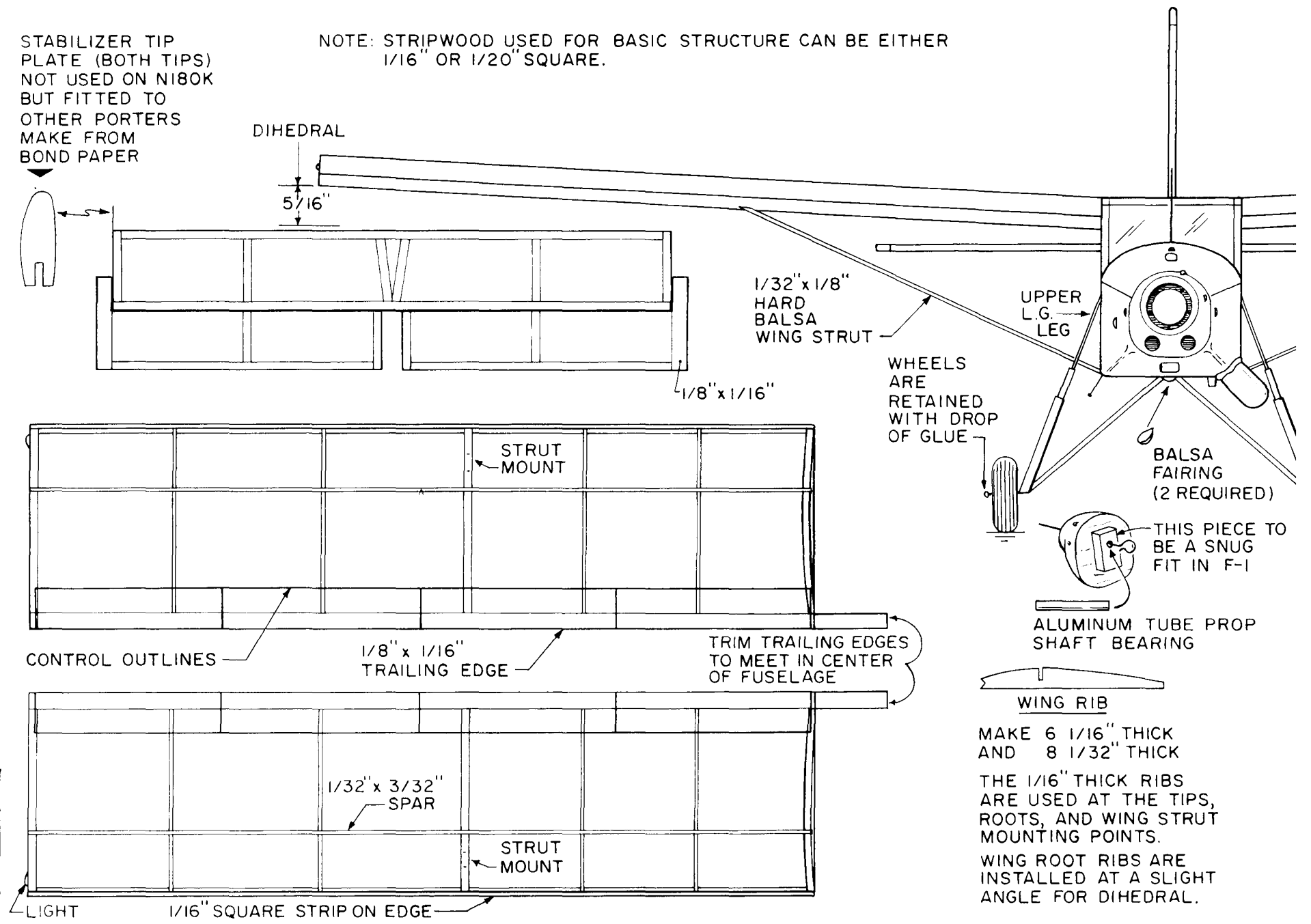
PILATUS TURBO-PEANUT TURBOMECA ASTAZOU ENGINE DRAWN BY W.C. HANNAN
