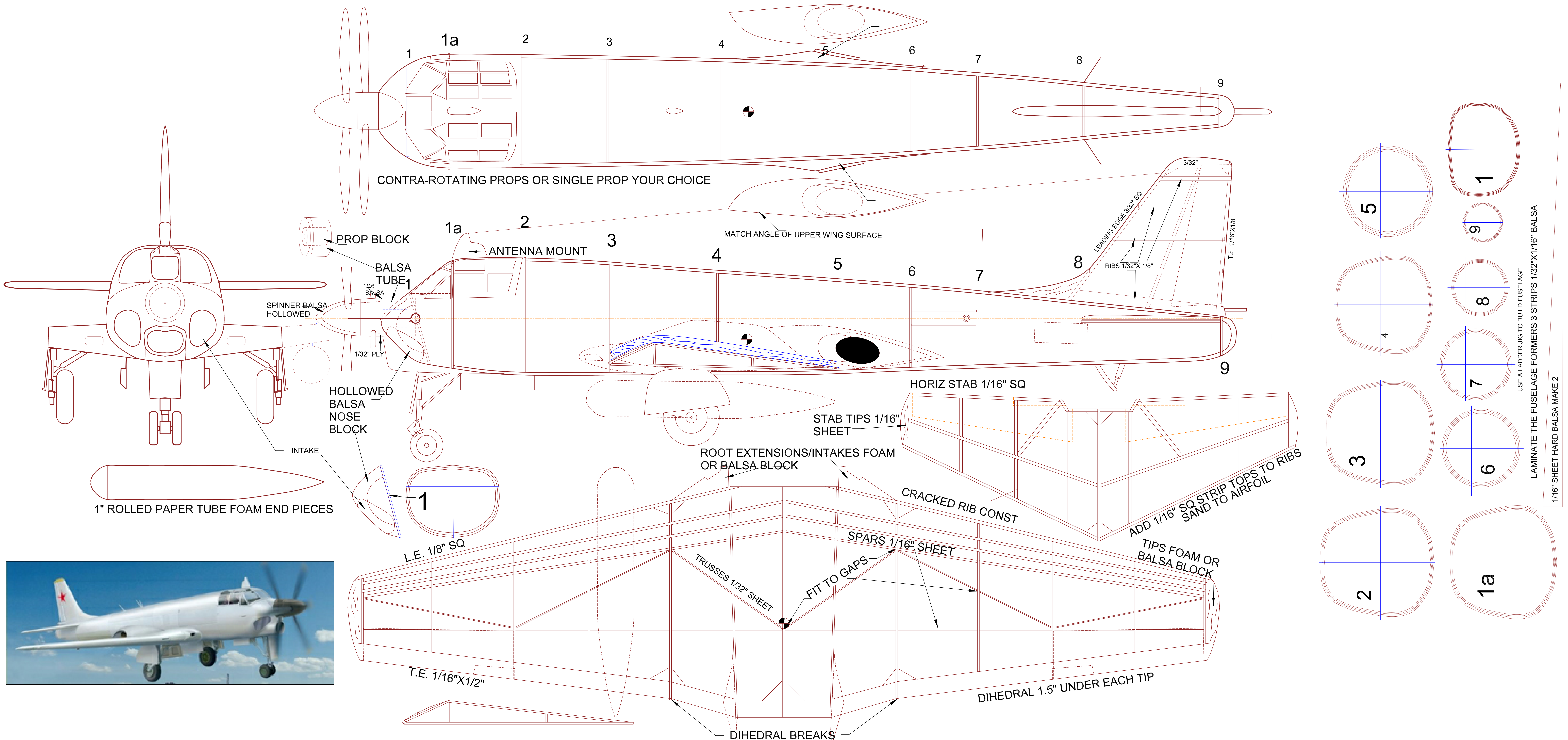
TUPOLEV TU-91 "BOOT" 27" SPAN DRAWN BY TOM AKERY 15 SEPT 23
