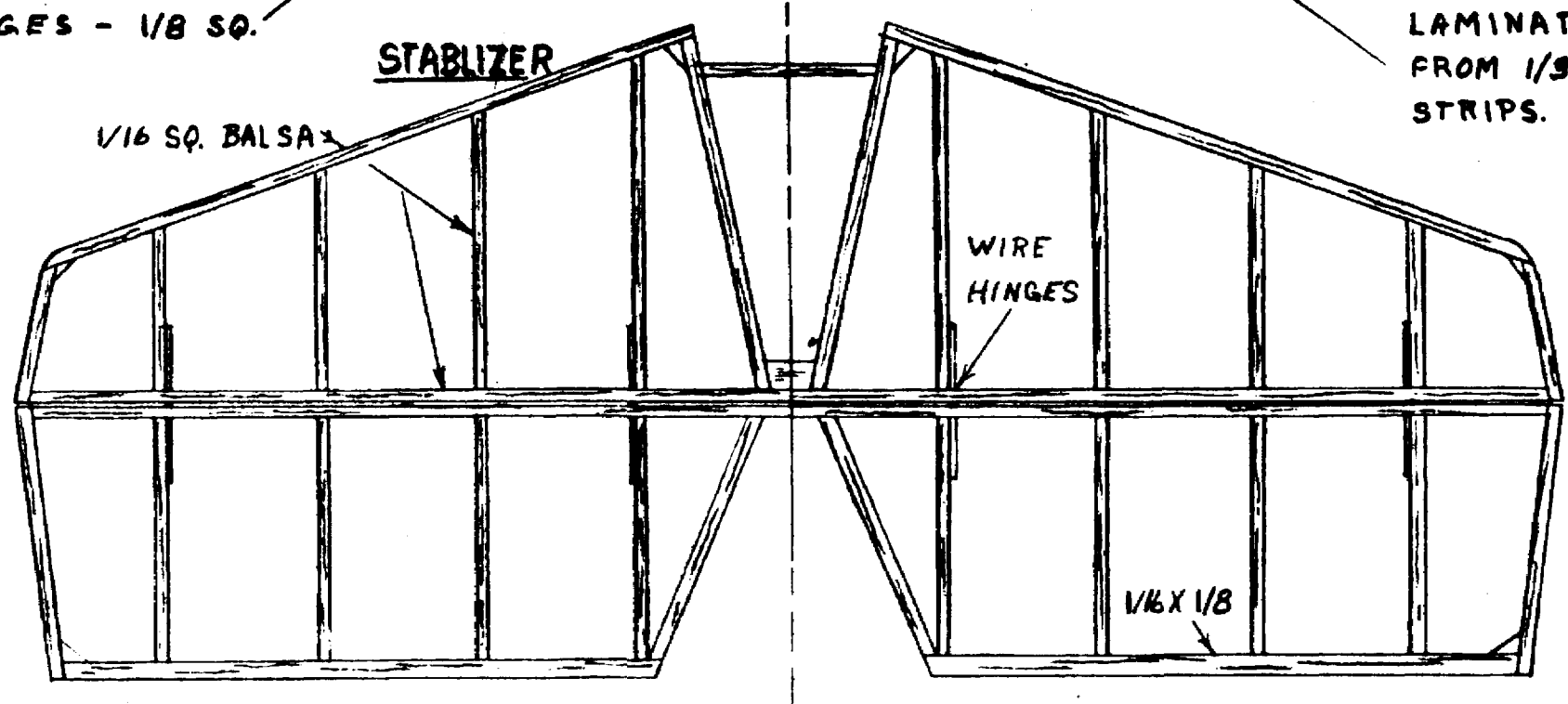
TOP VIEW
