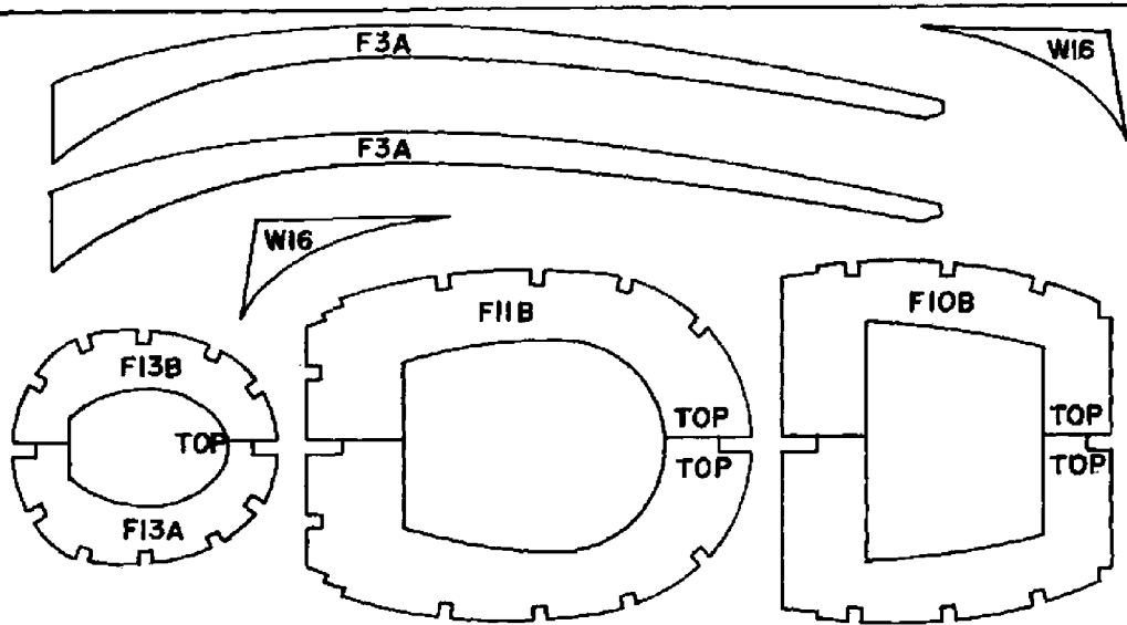
1/32" THICK Balsa
