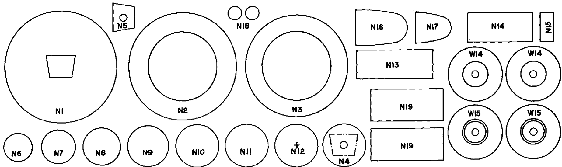
1/8" THICK Balsa
