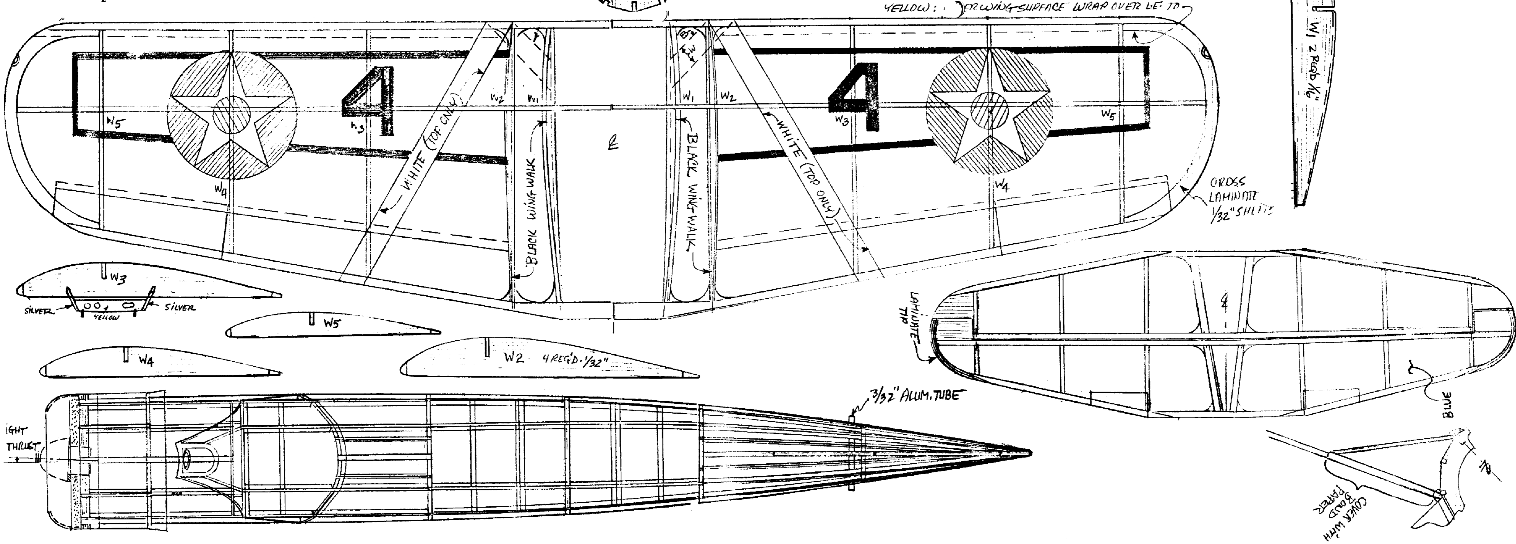
VOUGHT "KINGFISHER" by Pres Bruning Scale 1/2" = 1'
