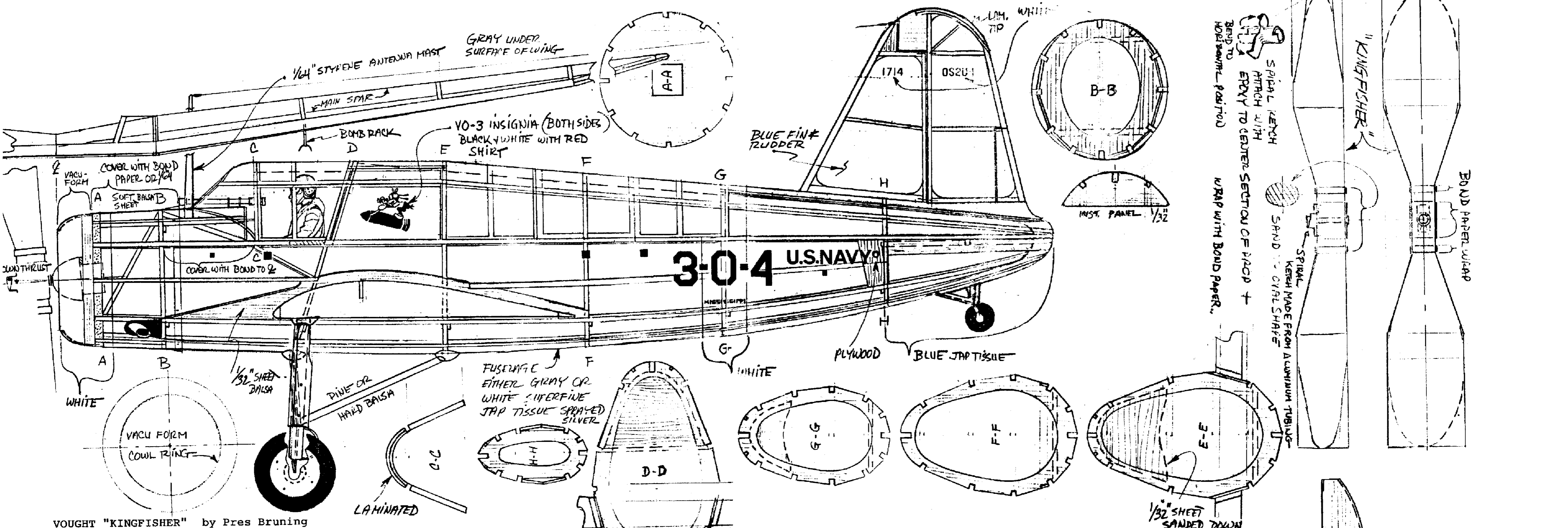
VOUGHT "KINGFISHER" by Pres Bruning Scale 1/2" = 1'
